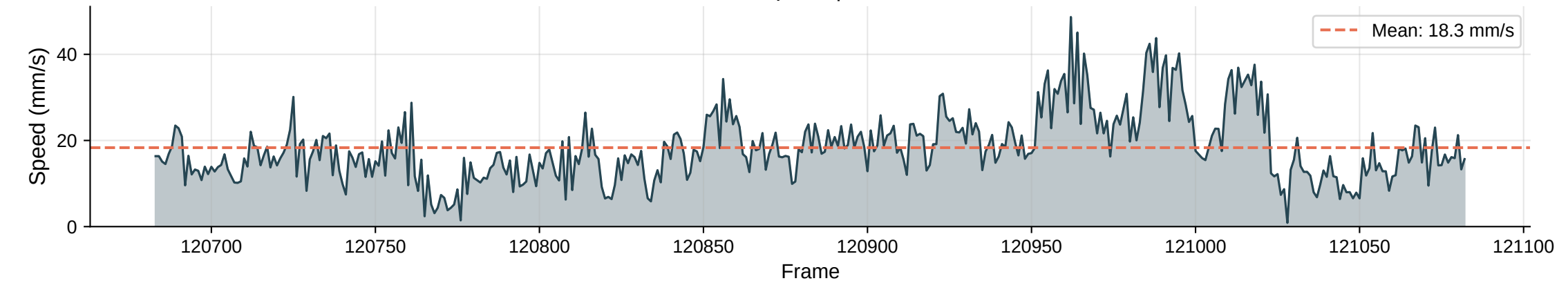
Instantaneous Speed | Max: 48.7 mm/s
