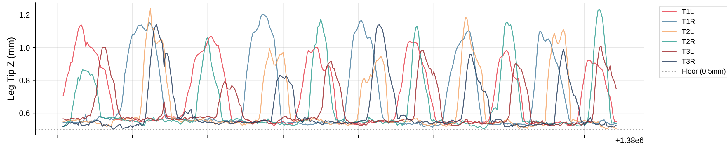
Leg Tip Z Trajectories | Bout 3
