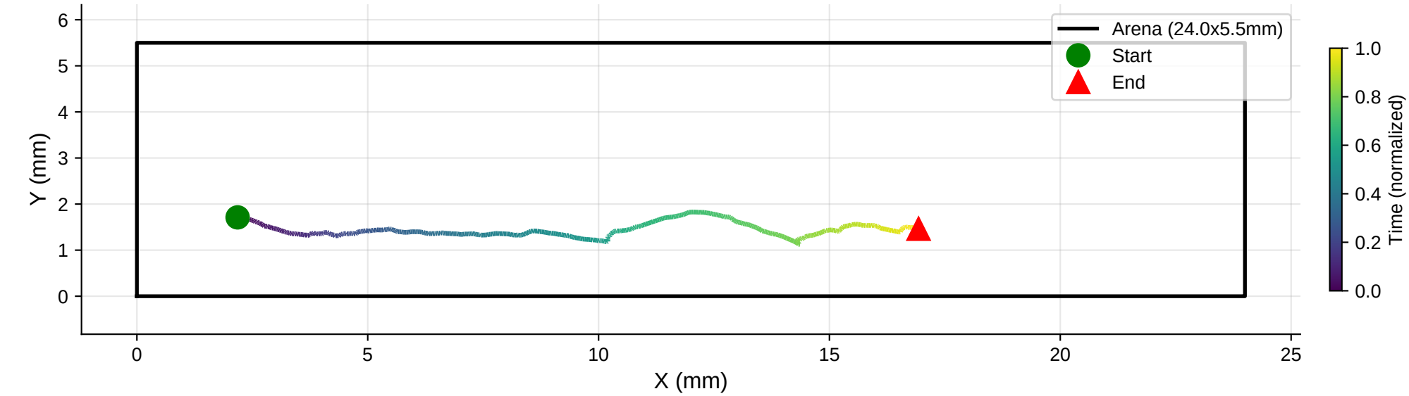
XY Trajectory | Distance: 15.86 mm
