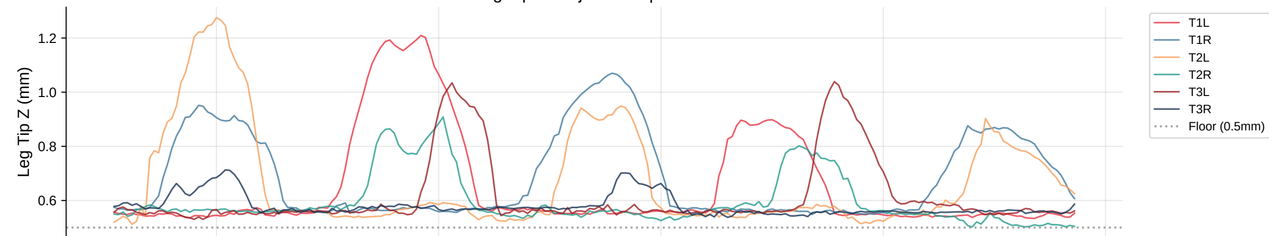
Leg Tip Z Trajectories | Bout 11
