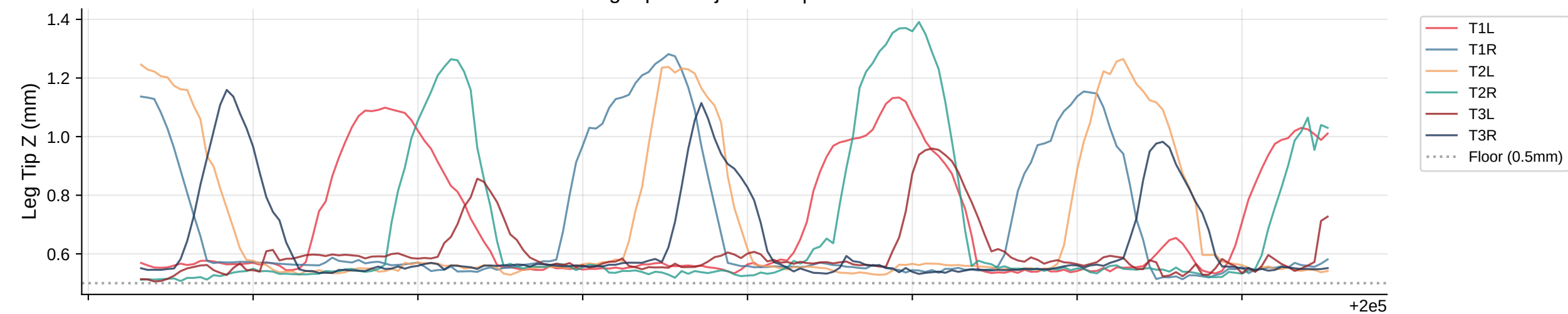
Leg Tip Z Trajectories | Bout 13
