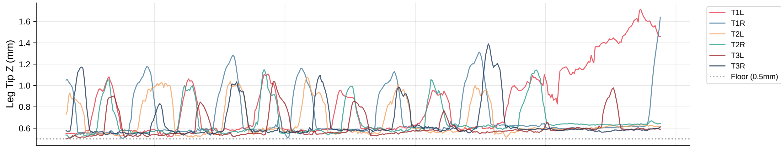
Leg Tip Z Trajectories | Bout 13
