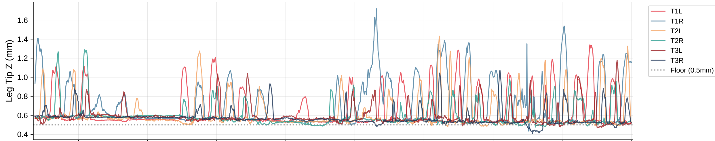
Leg Tip Z Trajectories | Bout 15
