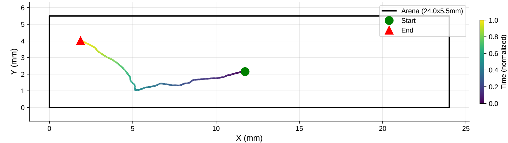
XY Trajectory | Distance: 11.60 mm
