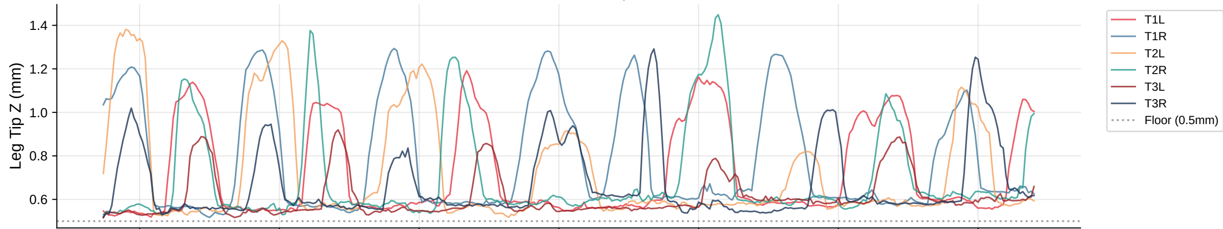
Leg Tip Z Trajectories | Bout 16
