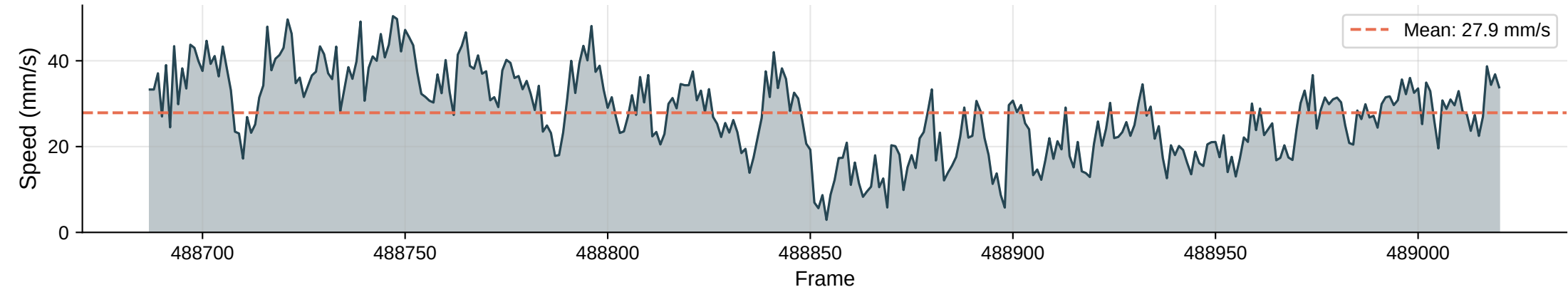
Instantaneous Speed | Max: 50.4 mm/s
