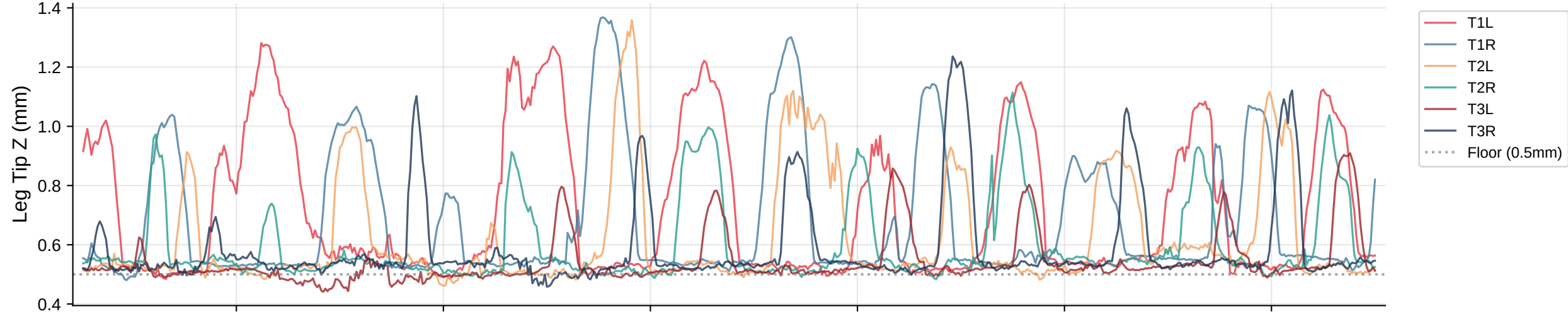
Leg Tip Z Trajectories | Bout 18
