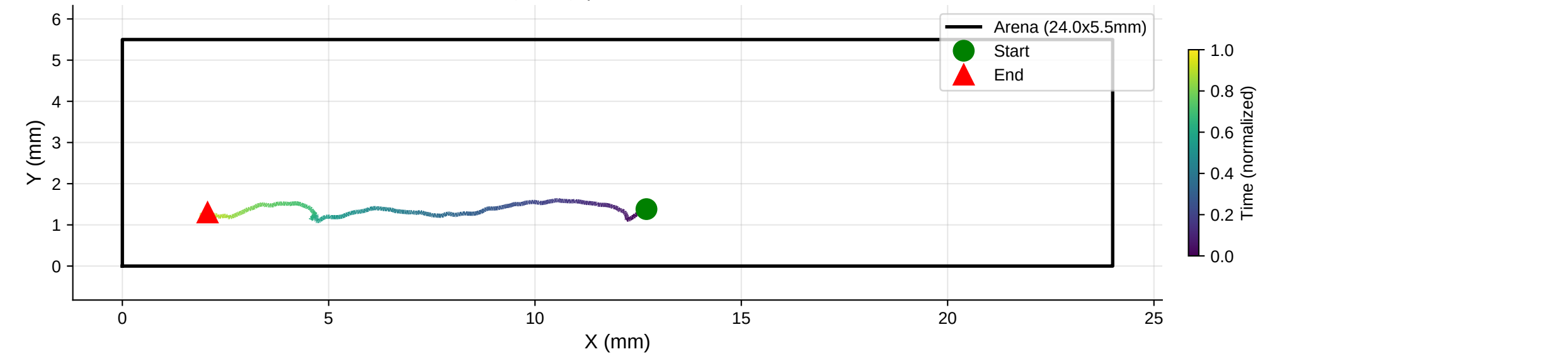
XY Trajectory | Distance: 12.73 mm
