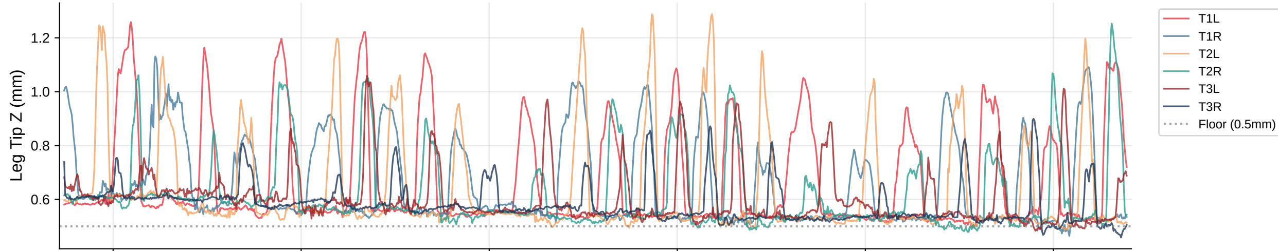
Leg Tip Z Trajectories | Bout 32
