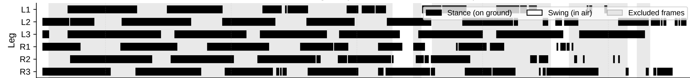
Gait Phase Diagram (black = stance, Z ? 0.59mm)
