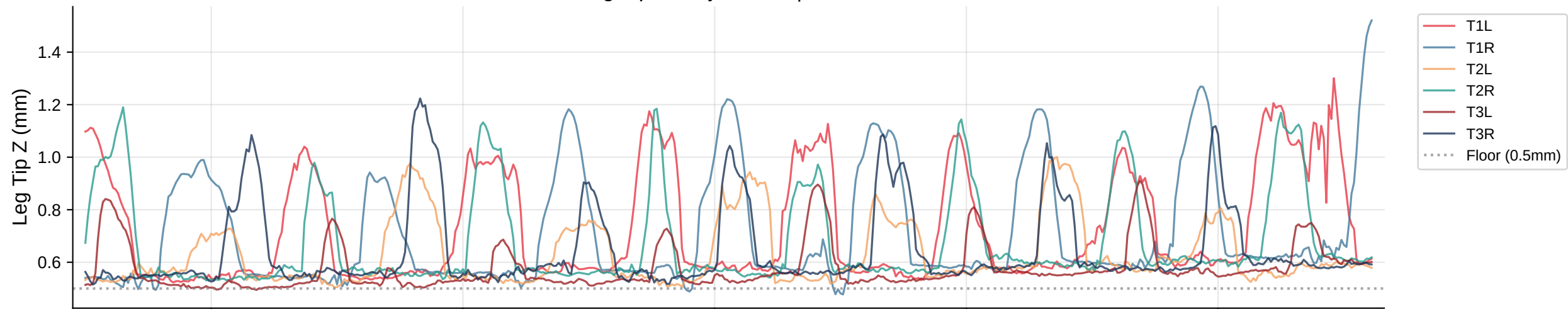
Leg Tip Z Trajectories | Bout 37
