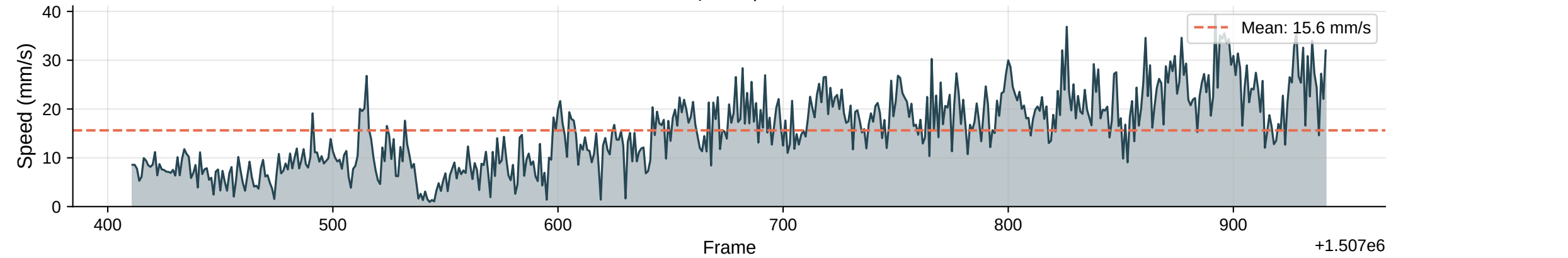
Instantaneous Speed | Max: 39.2 mm/s
