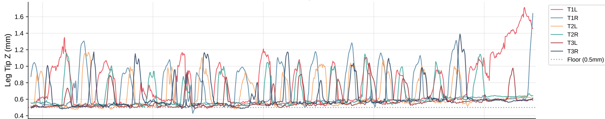
Leg Tip Z Trajectories | Bout 41
