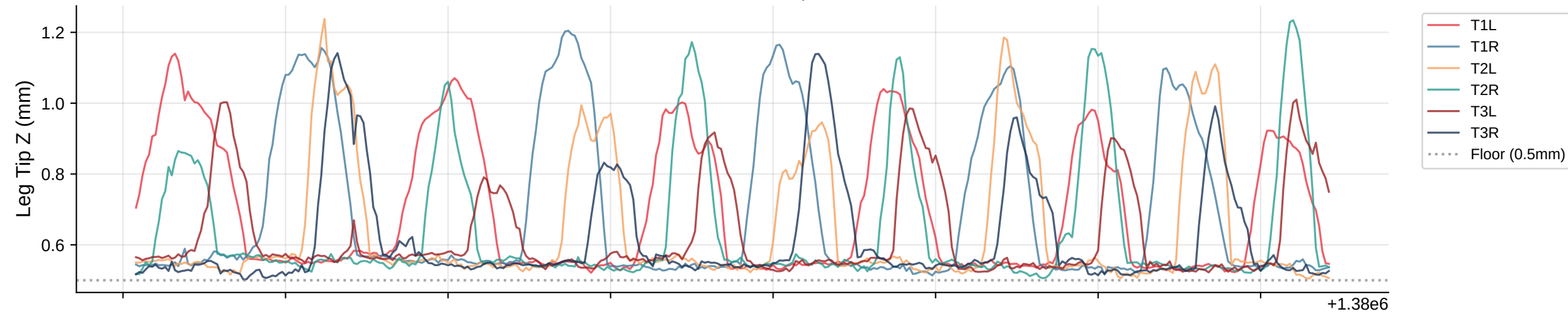
Leg Tip Z Trajectories | Bout 44
