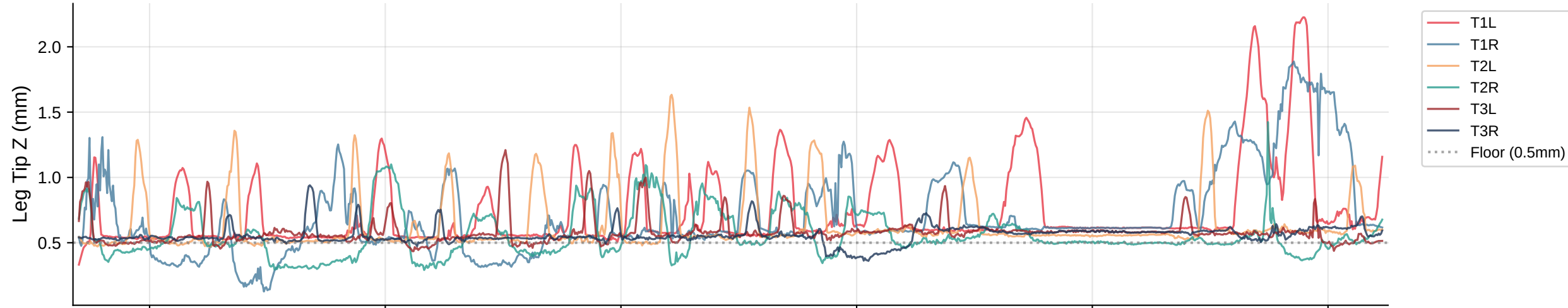
Leg Tip Z Trajectories | Bout 45
