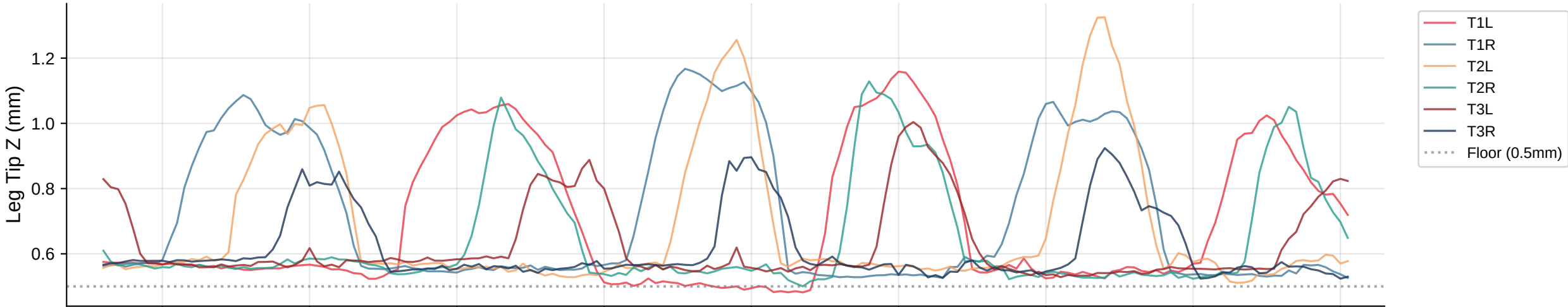
Leg Tip Z Trajectories | Bout 48
