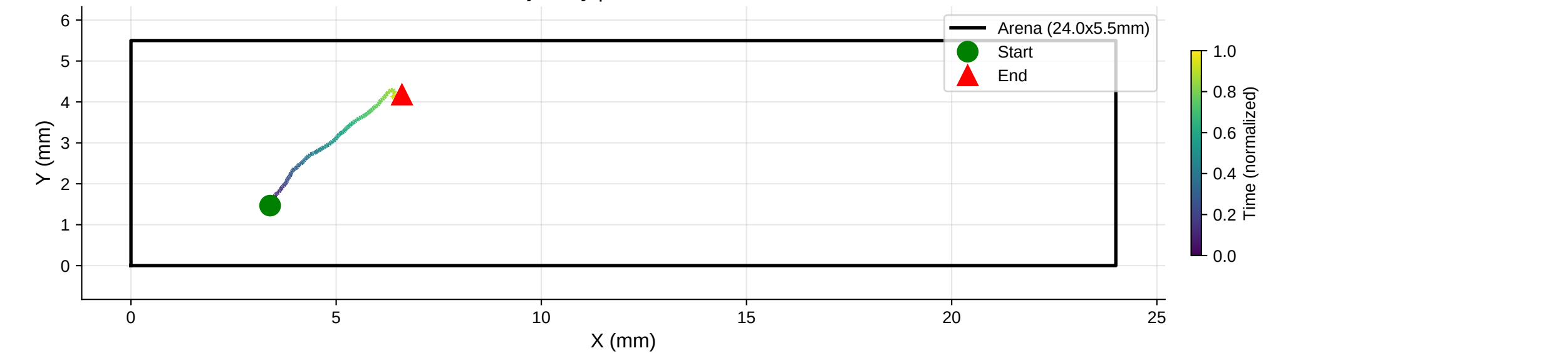
XY Trajectory | Distance: 5.01 mm
