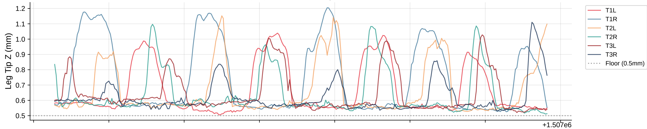
Leg Tip Z Trajectories | Bout 50
