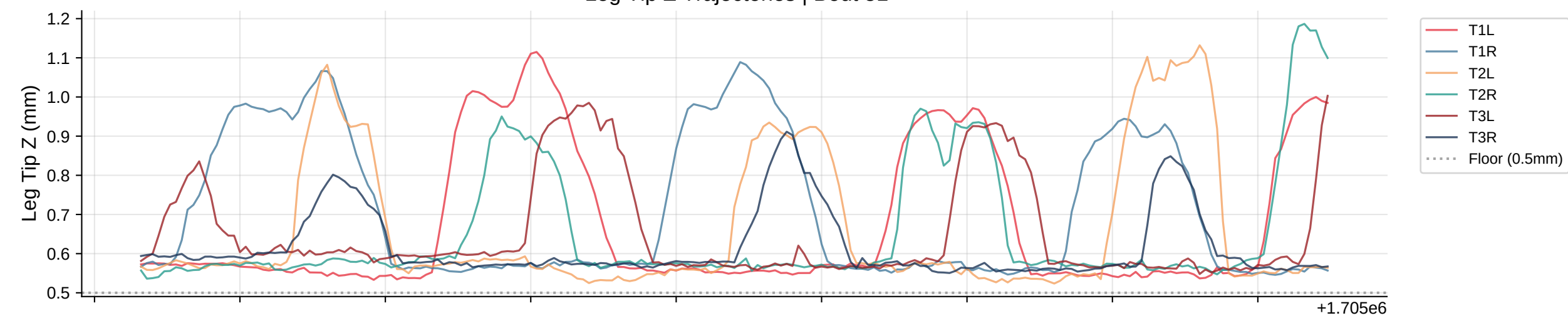
Leg Tip Z Trajectories | Bout 51
