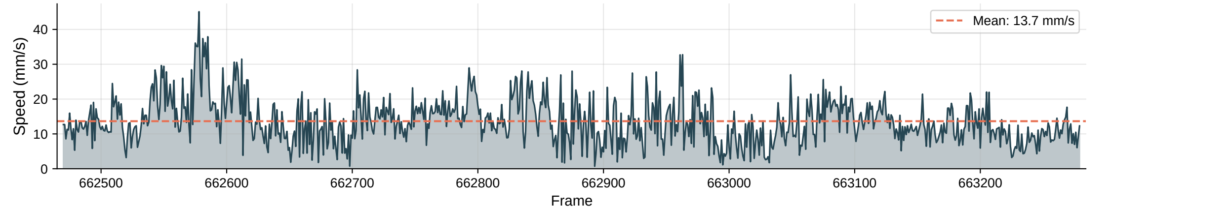
Instantaneous Speed | Max: 45.1 mm/s
