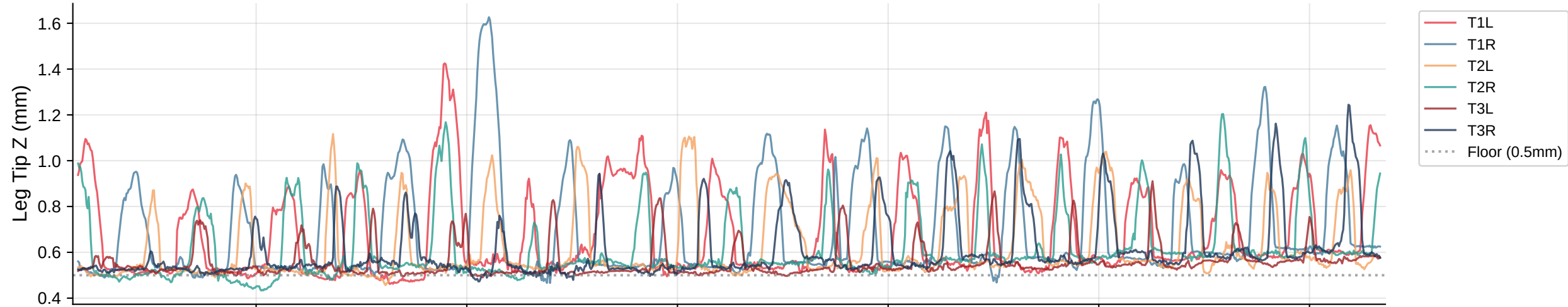
Leg Tip Z Trajectories | Bout 65
