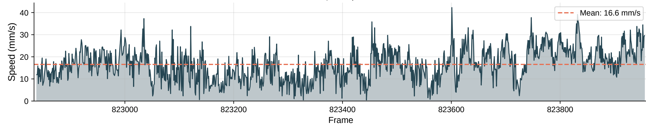
Instantaneous Speed | Max: 42.3 mm/s
