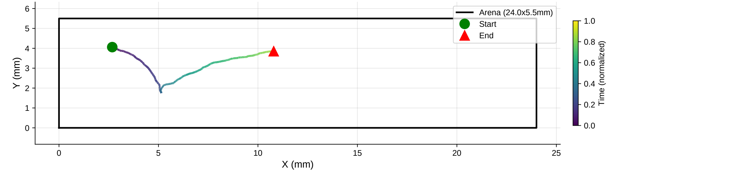
XY Trajectory | Distance: 10.84 mm
