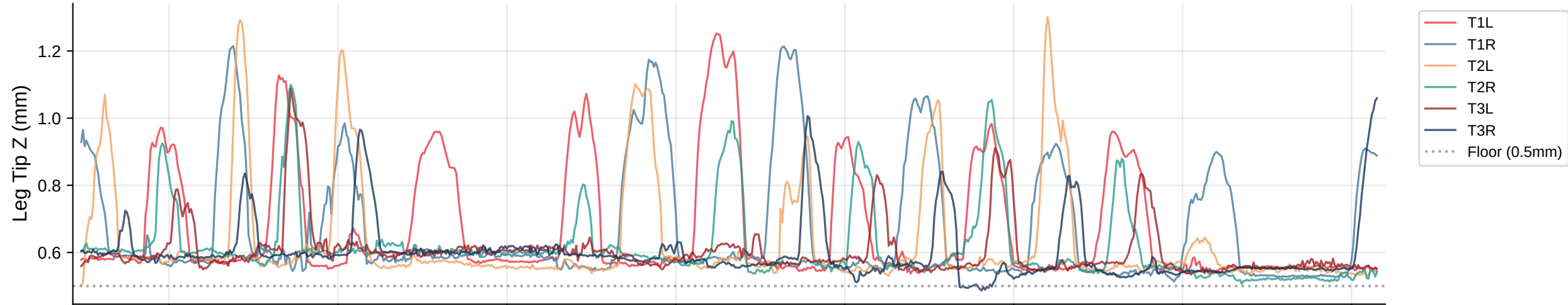
Leg Tip Z Trajectories | Bout 77
