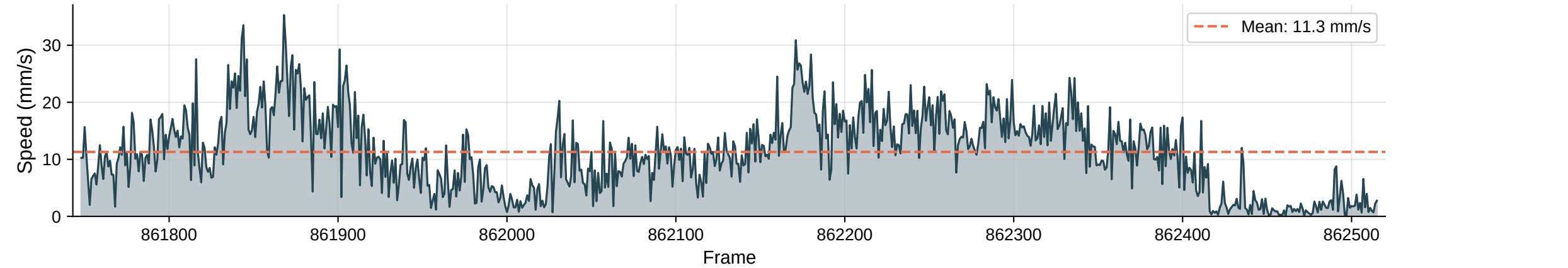
Instantaneous Speed | Max: 35.3 mm/s
