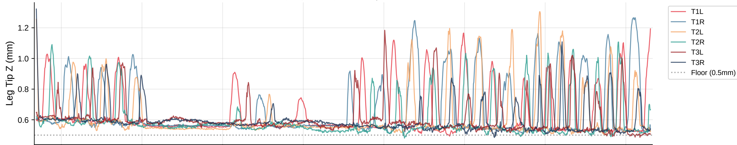
Leg Tip Z Trajectories | Bout 79
