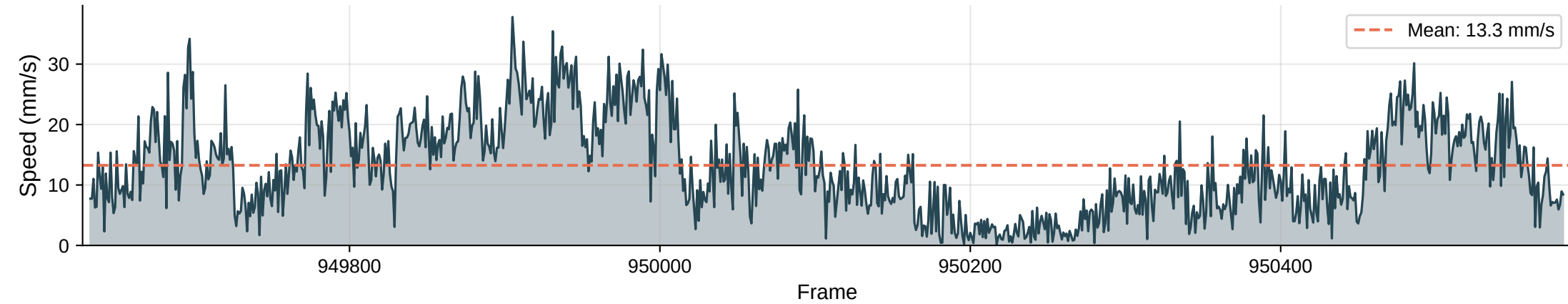
Instantaneous Speed | Max: 37.8 mm/s
