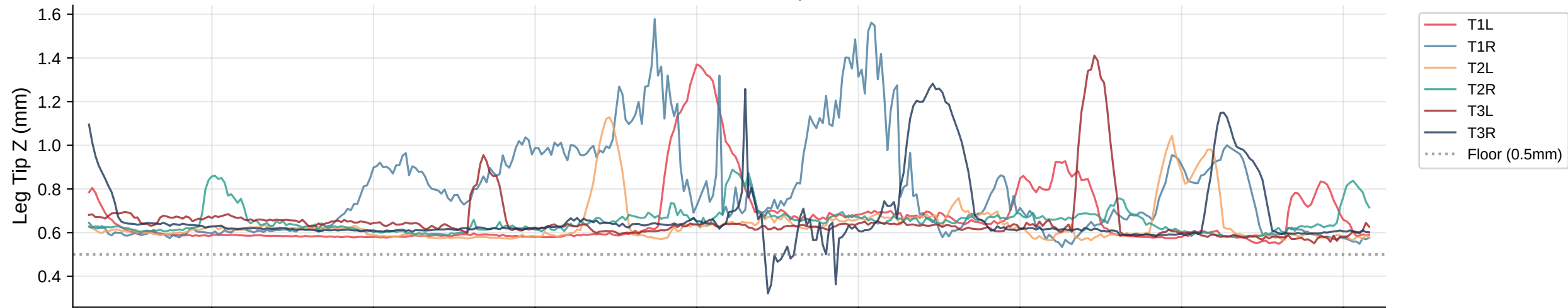
Leg Tip Z Trajectories | Bout 86
