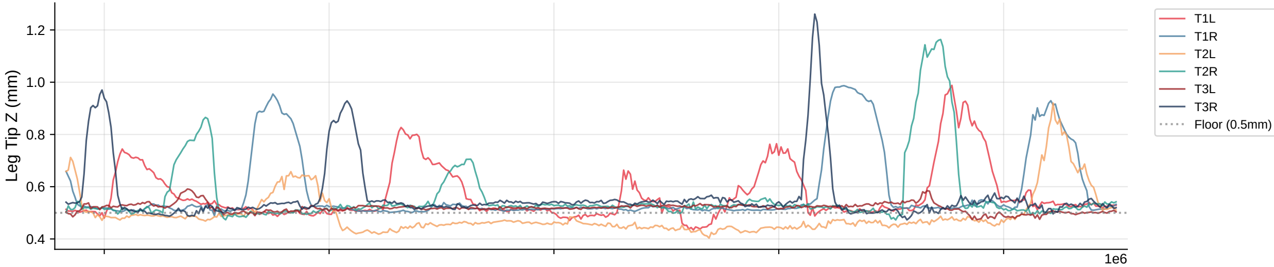
Leg Tip Z Trajectories | Bout 89
