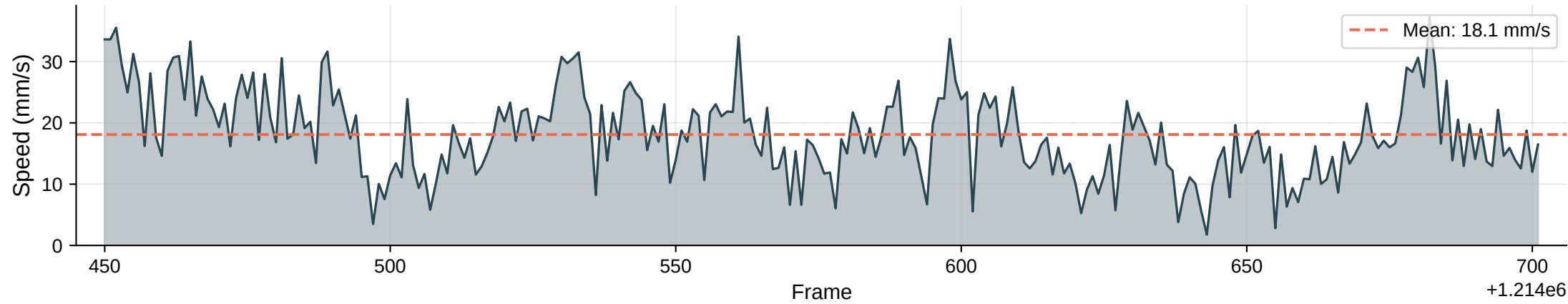
Instantaneous Speed | Max: 37.3 mm/s
