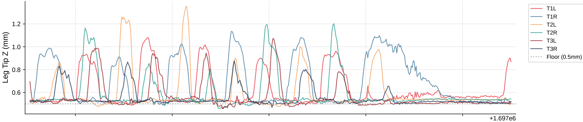
Leg Tip Z Trajectories | Bout 126
