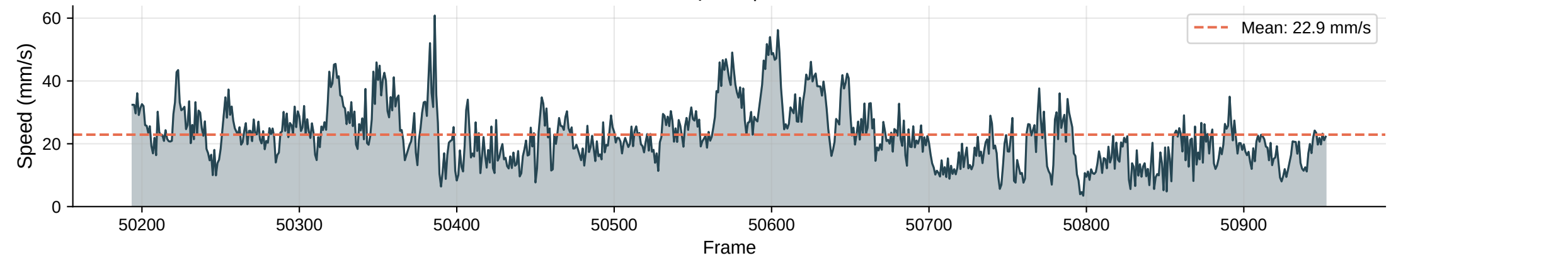
Instantaneous Speed | Max: 60.8 mm/s
