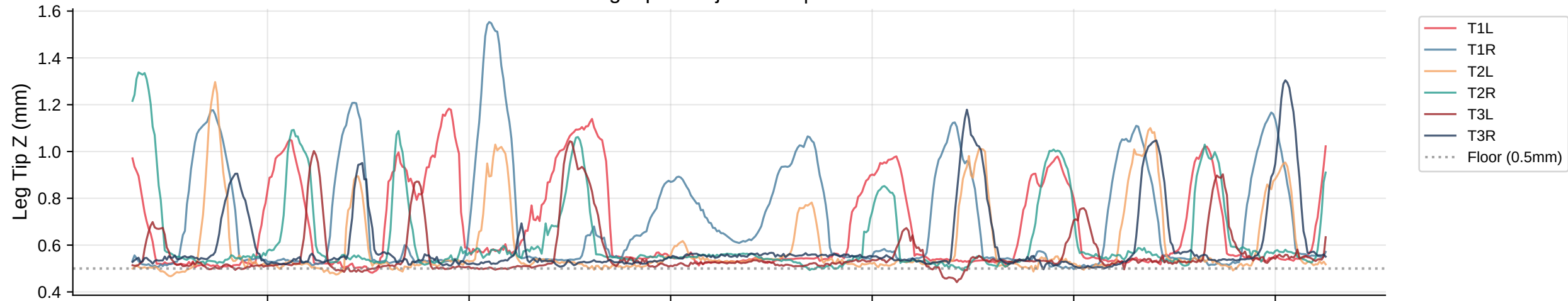
Leg Tip Z Trajectories | Bout 8
