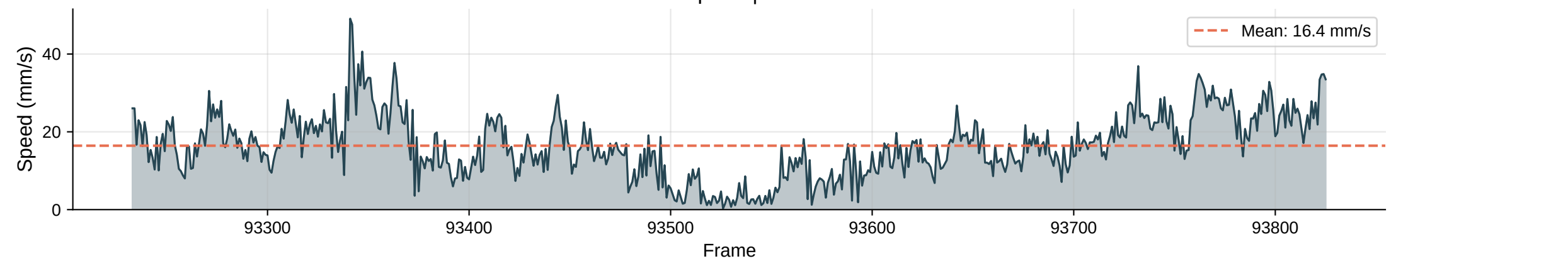
Instantaneous Speed | Max: 49.1 mm/s
