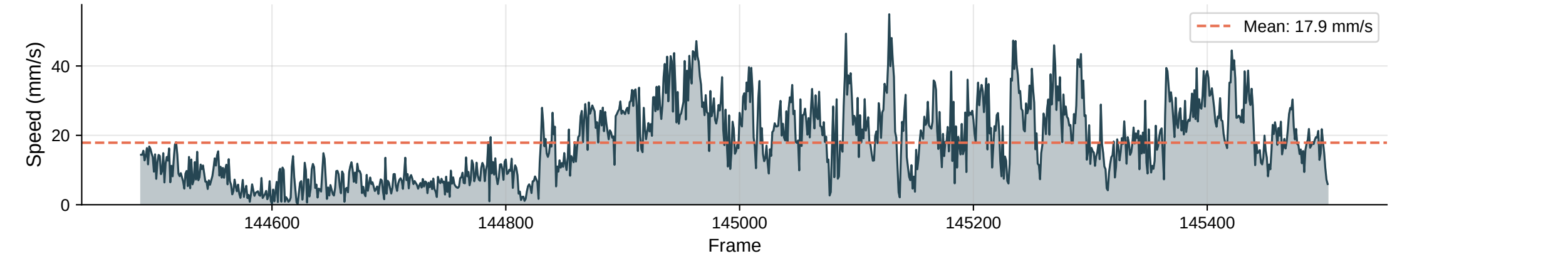
Instantaneous Speed | Max: 54.9 mm/s
