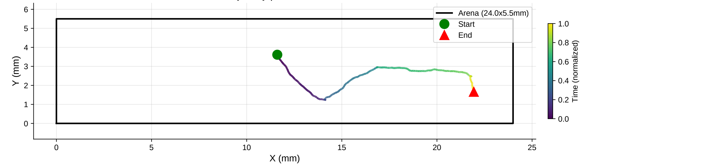
XY Trajectory | Distance: 14.62 mm
