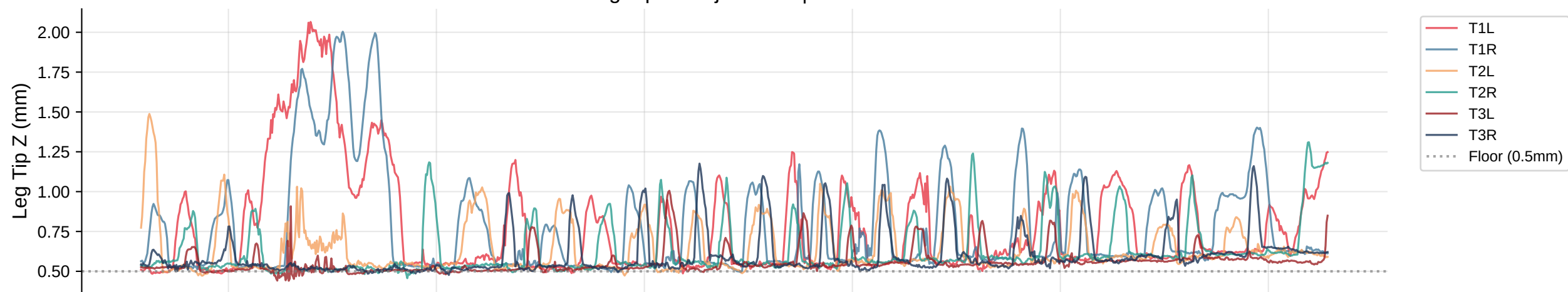
Leg Tip Z Trajectories | Bout 21
