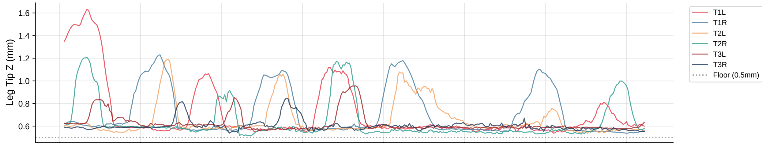
Leg Tip Z Trajectories | Bout 22
