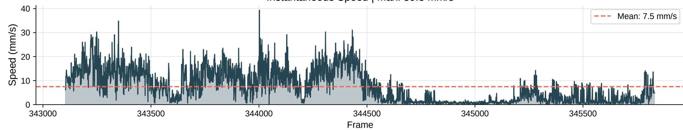
Instantaneous Speed | Max: 39.3 mm/s
