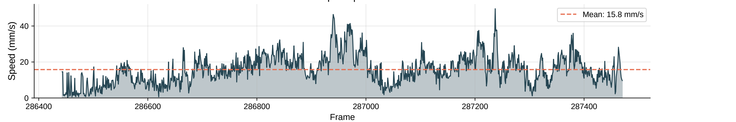
Instantaneous Speed | Max: 49.6 mm/s
