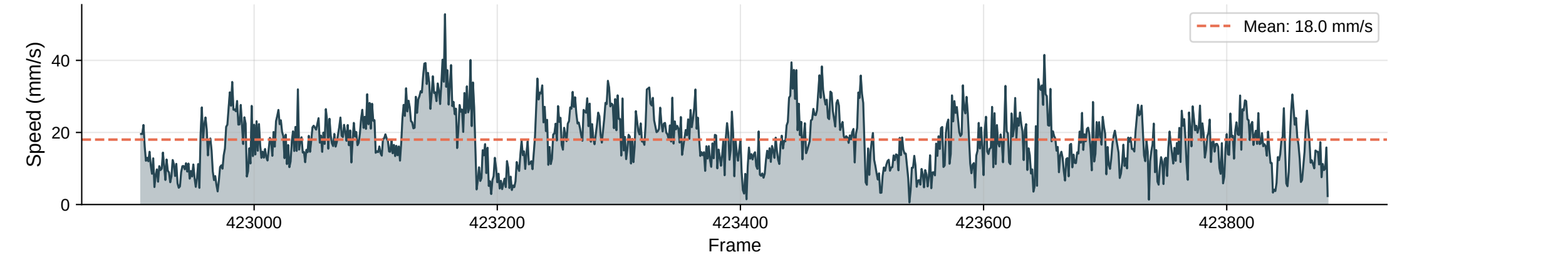
Instantaneous Speed | Max: 52.8 mm/s
