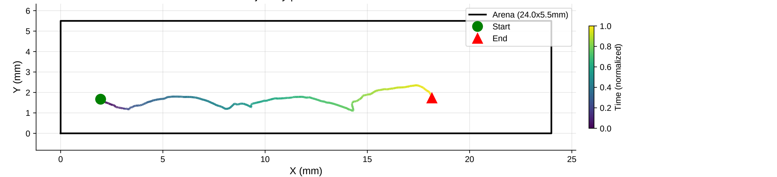
XY Trajectory | Distance: 18.42 mm
