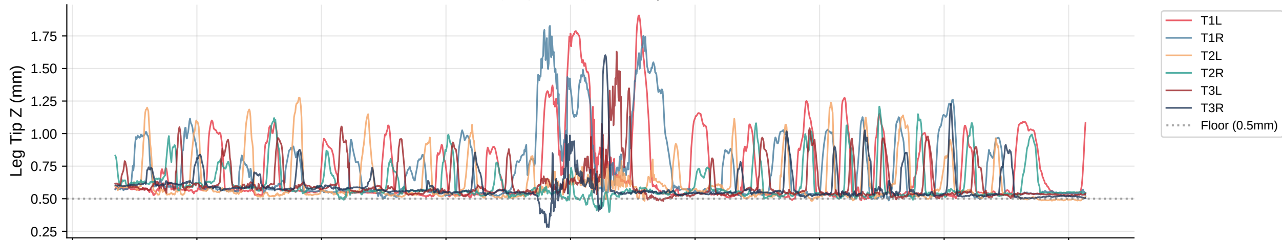
Leg Tip Z Trajectories | Bout 40
