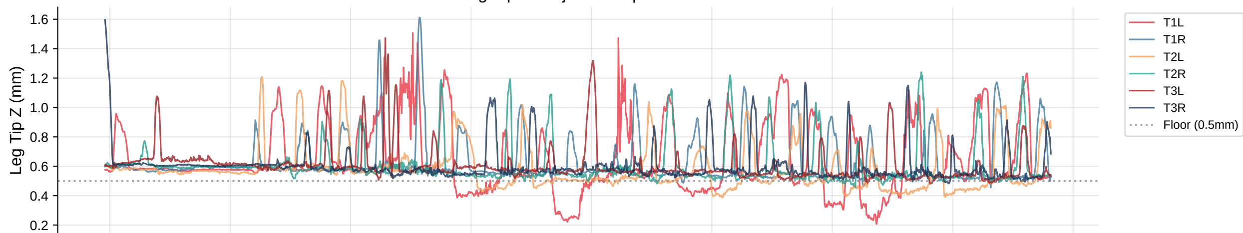
Leg Tip Z Trajectories | Bout 43
