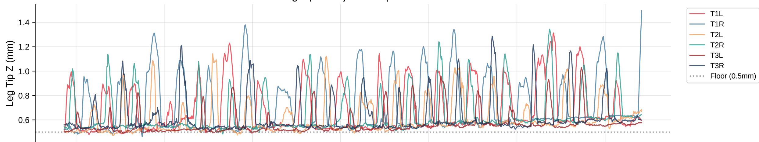
Leg Tip Z Trajectories | Bout 52
