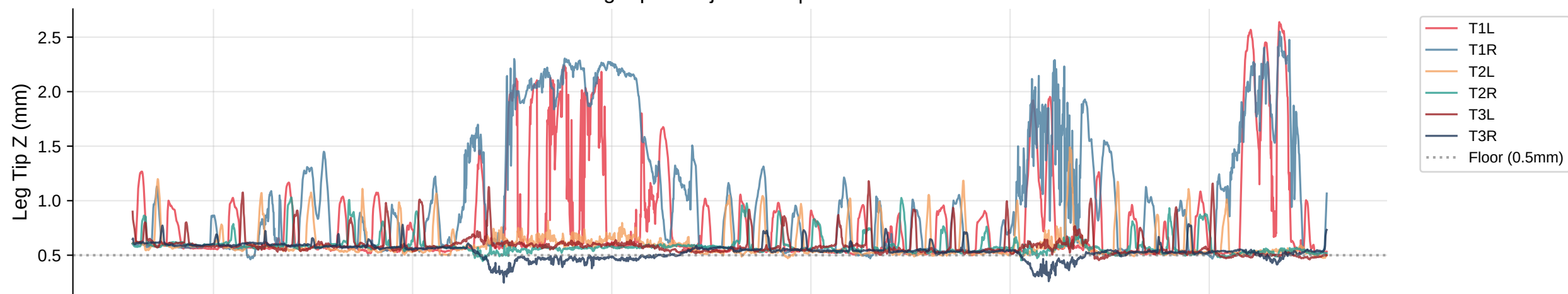
Leg Tip Z Trajectories | Bout 53
