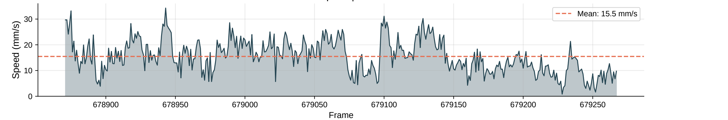
Instantaneous Speed | Max: 34.3 mm/s
