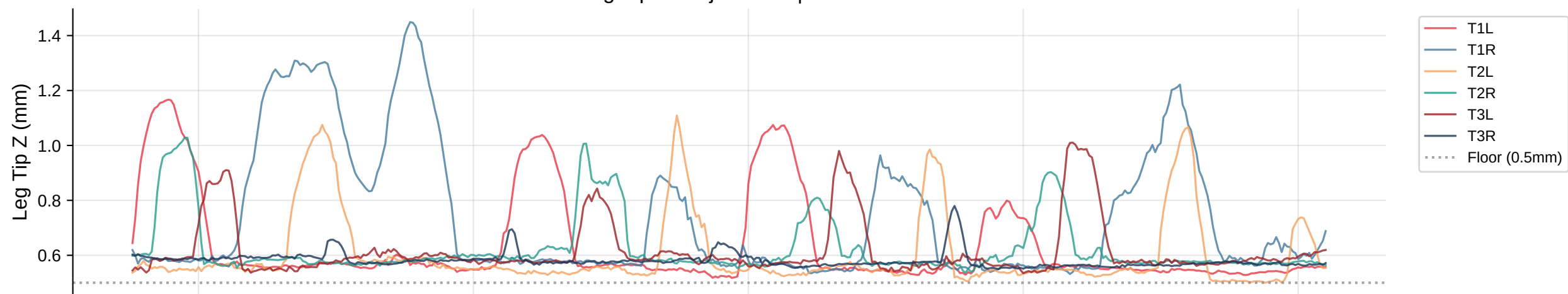
Leg Tip Z Trajectories | Bout 60
