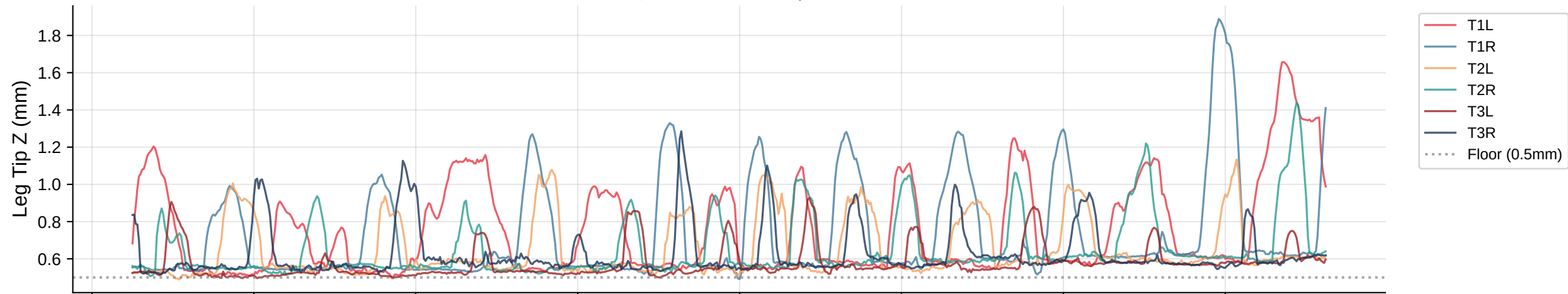
Leg Tip Z Trajectories | Bout 62
