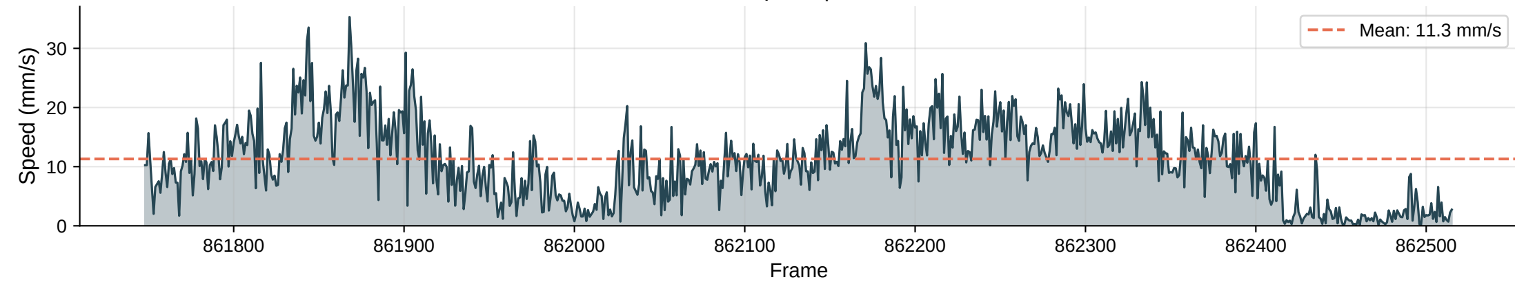
Instantaneous Speed | Max: 35.3 mm/s
