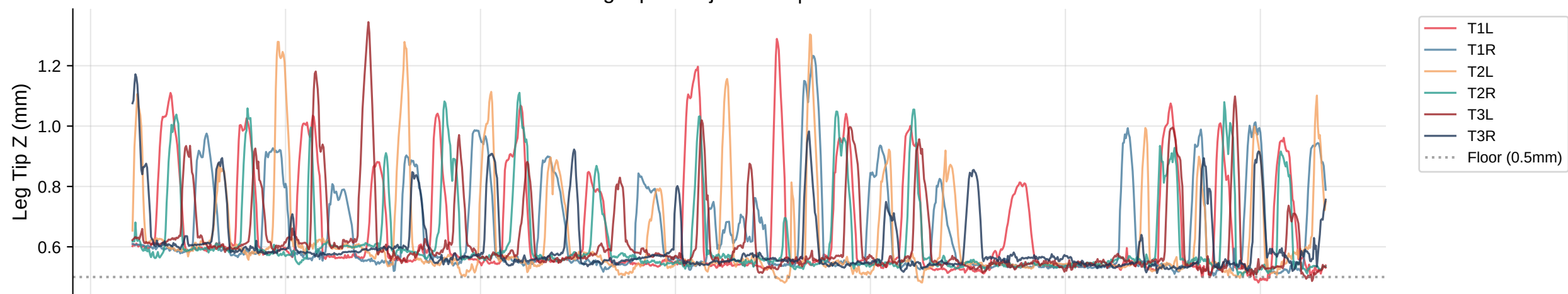
Leg Tip Z Trajectories | Bout 63
