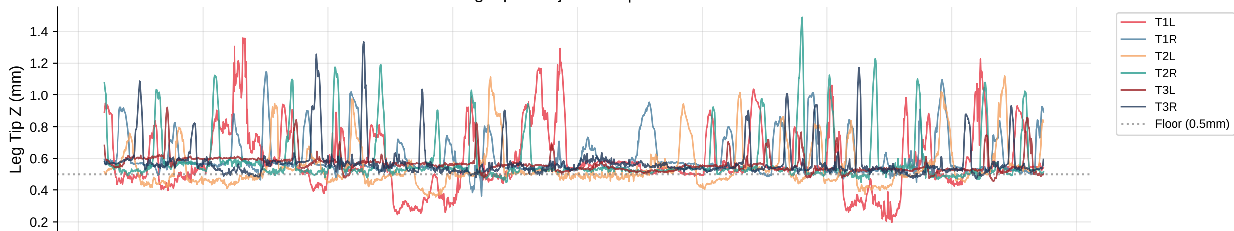
Leg Tip Z Trajectories | Bout 65
